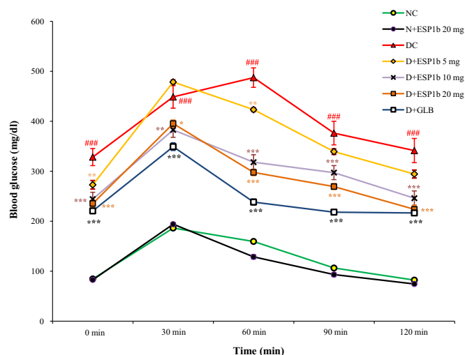
Fig. 2. Effect of ESP1b on blood glucose levels during the oral glucose tolerance test in normal and streptozotocin-induced diabetic Wistar rats. NC, Normal control rats; N+ESP1b 20 mg, Normal rats treated with high dose of ESP1b (20 mg/kg b.w./day); DC, STZ-induced diabetic control rats; D+ESP1b 5 mg, STZ-induced diabetic rats treated with low dose of ESP1b (5 mg/kg b.w./day); D+ESP1b 10 mg, STZ-induced diabetic rats treated with medium dose of ESP1b (10 mg/kg b.w./day); D+ESP1b 20 mg, STZ-induced diabetic rats treated with high dose of ESP1b (20 mg/kg b.w./day); and D+GLB, STZ-induced diabetic rats treated with glibenclamide (600 \mu\text{g/kg} b.w./day). Values are mean \pm S.E.M. (n=6). * P < 0.05 , ** P < 0.01 , *** P < 0.001 compared to NC group. * P < 0.05 , ** P < 0.01 , *** P < 0.001 compared to DC group.
