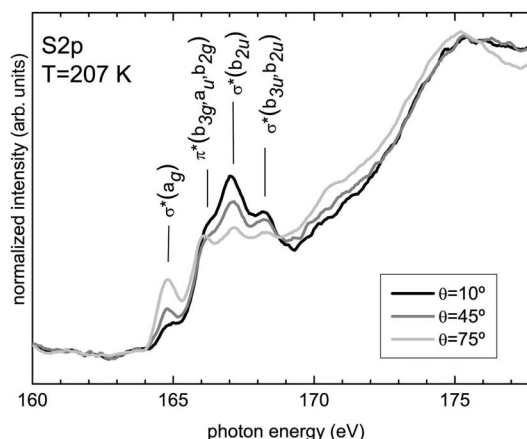
FIG. 3. Normalized S 2 p XANES spectra for (TMTTF) 2 ReO 4 taken at 207 K for \theta=10^\circ (solid black line), 45^\circ (solid gray line) and 75^\circ (solid light gray line).
