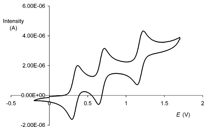
Figure 7. Cyclic voltammogram of TTF-DMA in CH_3CN , at room temperature, with 0.1 \text{ M nBu}_4\text{BF}_4 as supporting electrolyte (Pt electrode, r = 0.5 \text{ mm} ), scan rate = 0.1 \text{ V s}^{-1} . The E values are vs SCE.
