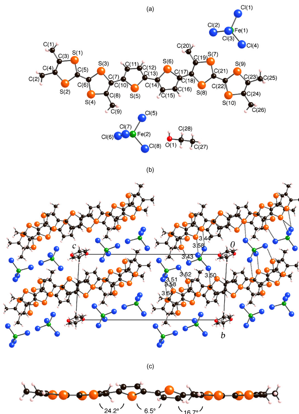
Fig. 2. (a) Crystallographically independent unit in the 3d(FeCl_4)_2(ethanol) salt, (b) crystal structure of the 3d(FeCl_4)_2(ethanol) salt projected to the bc plane, and (c) side view of the donor molecule 3d .
