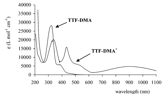
Figure 9. UV–visible electronic spectra of TTF-DMA and [\text{TTF-DMA}]^+ in acetonitrile.
