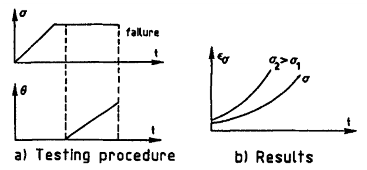
Figure 1.18 Essai Transitoire
