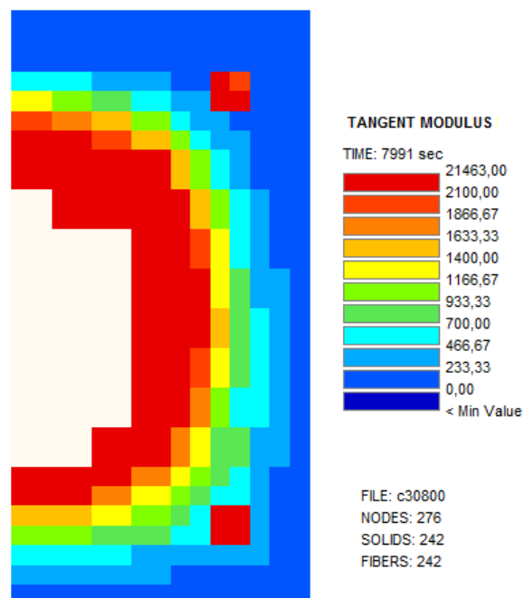
Figure 4 : Module tangent t = 133min11sec
