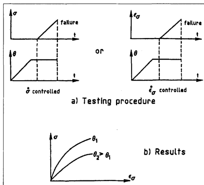
Figure 1.17 Essai stationnaire
