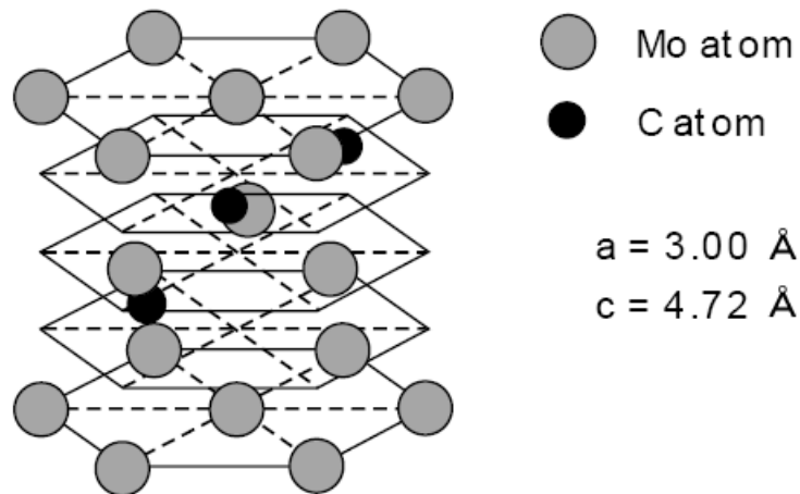
Figure 1.21. : Structure du carbure Mo_2C [18]
